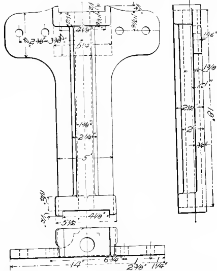
Figs. 4698-1700. BOLSTER GUIDE-BAR OR COLUMN.
